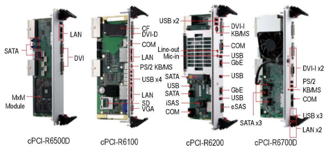
cPCI-R6500D
